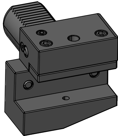
90 DEGREE VDI40 STATIC TOOL OUTPUT: 25mm SQR SHANK COOLANT: EXTERNAL
